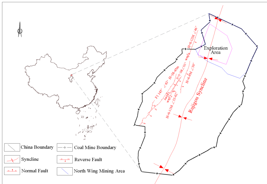
Figure 8. Schematic location map of the north wing mining area of baijigou coal mine
