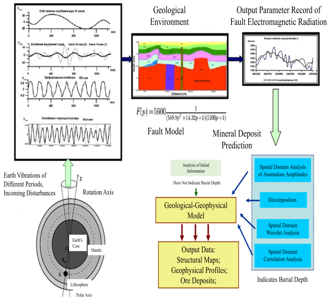
Figure 1 Schematic diagram of GPTS technology principle
