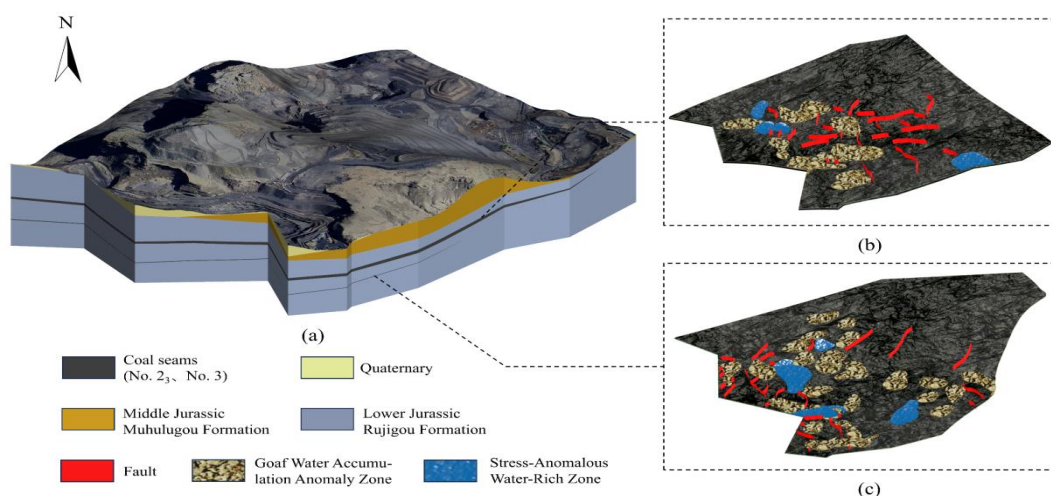
Figure 10. 3D geological model of the study area: (a) North wing mining panel model; (b) 3D model map of No. 23; (c) 3D model map of No. 3.
