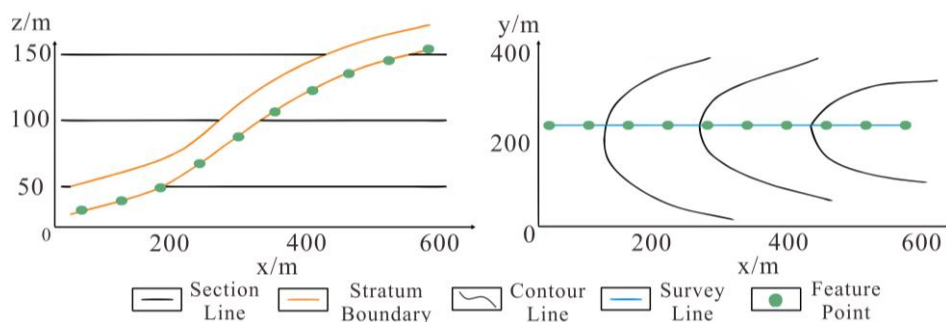
Figure 6. Schematic diagram of cross-sectional-to-planar projection technology
