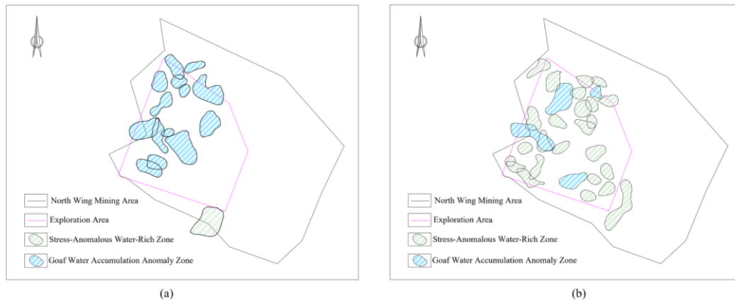
Figure 9. Exploration results map of the study area: (a)No. 23; (b)No.3.
